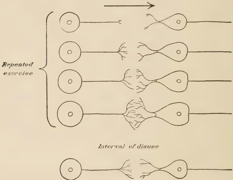
FIG. 3. The Law of Exercise in terms of synapses. The diagram shows four stages of a synapse as it is more and more closely connected through successful exercise and a fifth where the connection has, through disuse, grown less strong. (Adapted from Woodworth, Psychology , Holt, New York, 1921, p. 415.)
